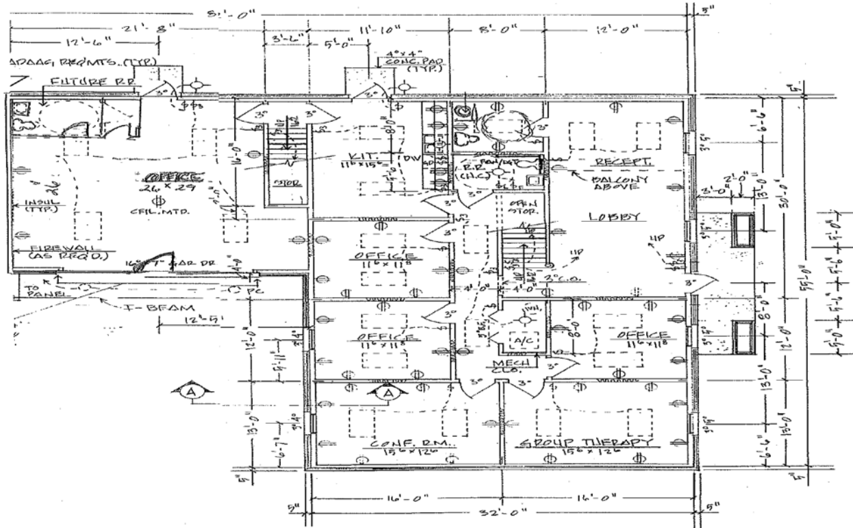
FLOOR PLAN - 1ST LEVEL SCALE: 1/8" = 1'-0"
