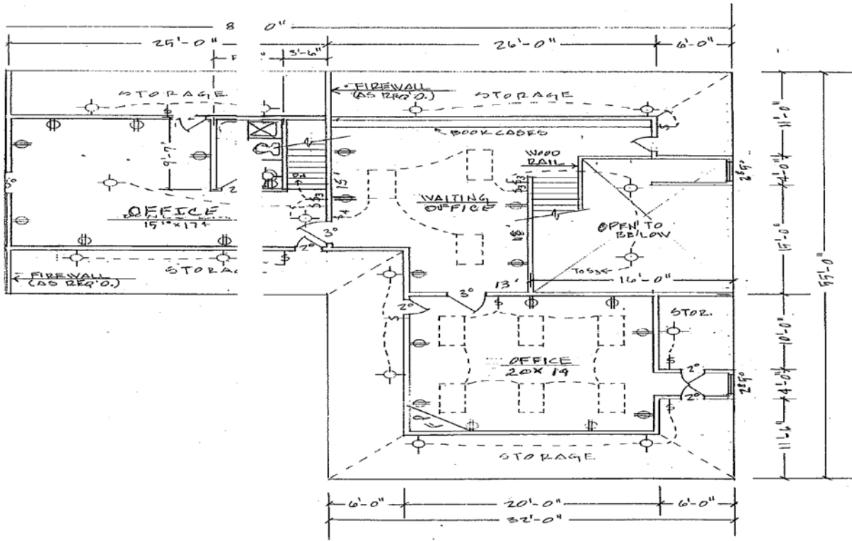
FLOOR PLAN - 2ND LEVEL SCALE: 1/8" = 1'-0"
